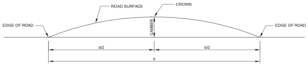
CAMBER OR CROSS-FALL OF ROAD SURFACE
