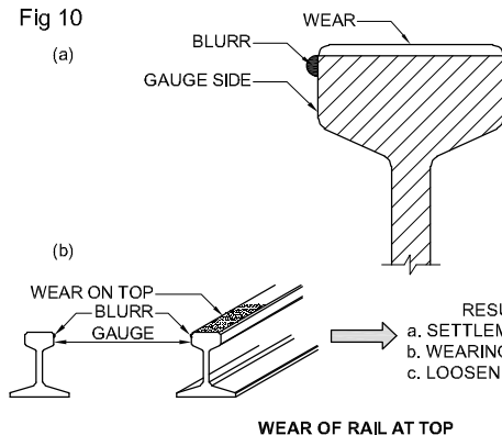
WEAR OF RAIL AT TOP
