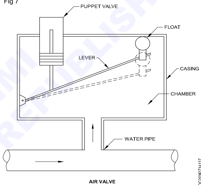
AIR VALVE
