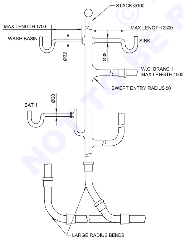
SINGLE STACK SYSTEM
