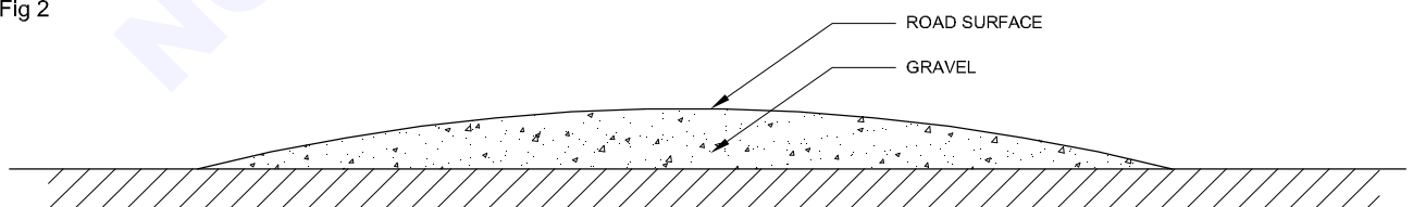
FEATHER EDGE TYPE CONSTRUCTION OF GRAVEL ROAD
