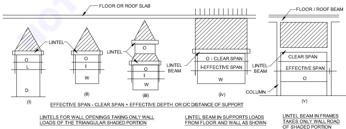
(a) LOAD ACTING ON LINTELS
