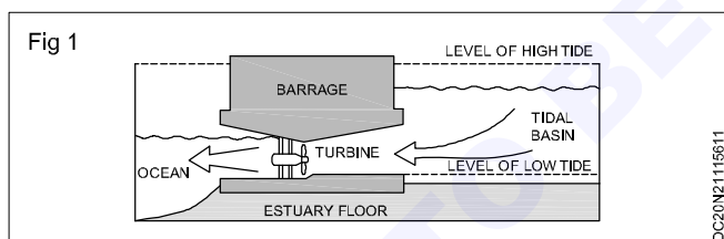
Fuction of a Barrage (Fig 2)
