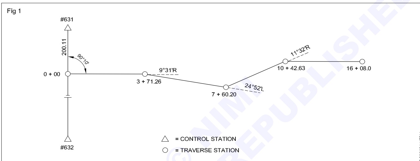
Figure 1: Open traverse
