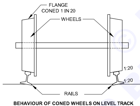
BEHAVIOUR OF CONED WHEELS ON LEVEL TRACK
