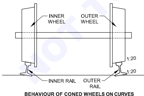
BEHAVIOUR OF CONED WHEELS ON CURVES
