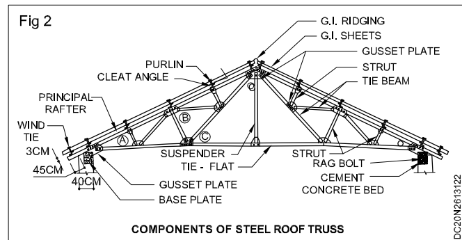
Details of the components of steel roof truss (Fig 2)
