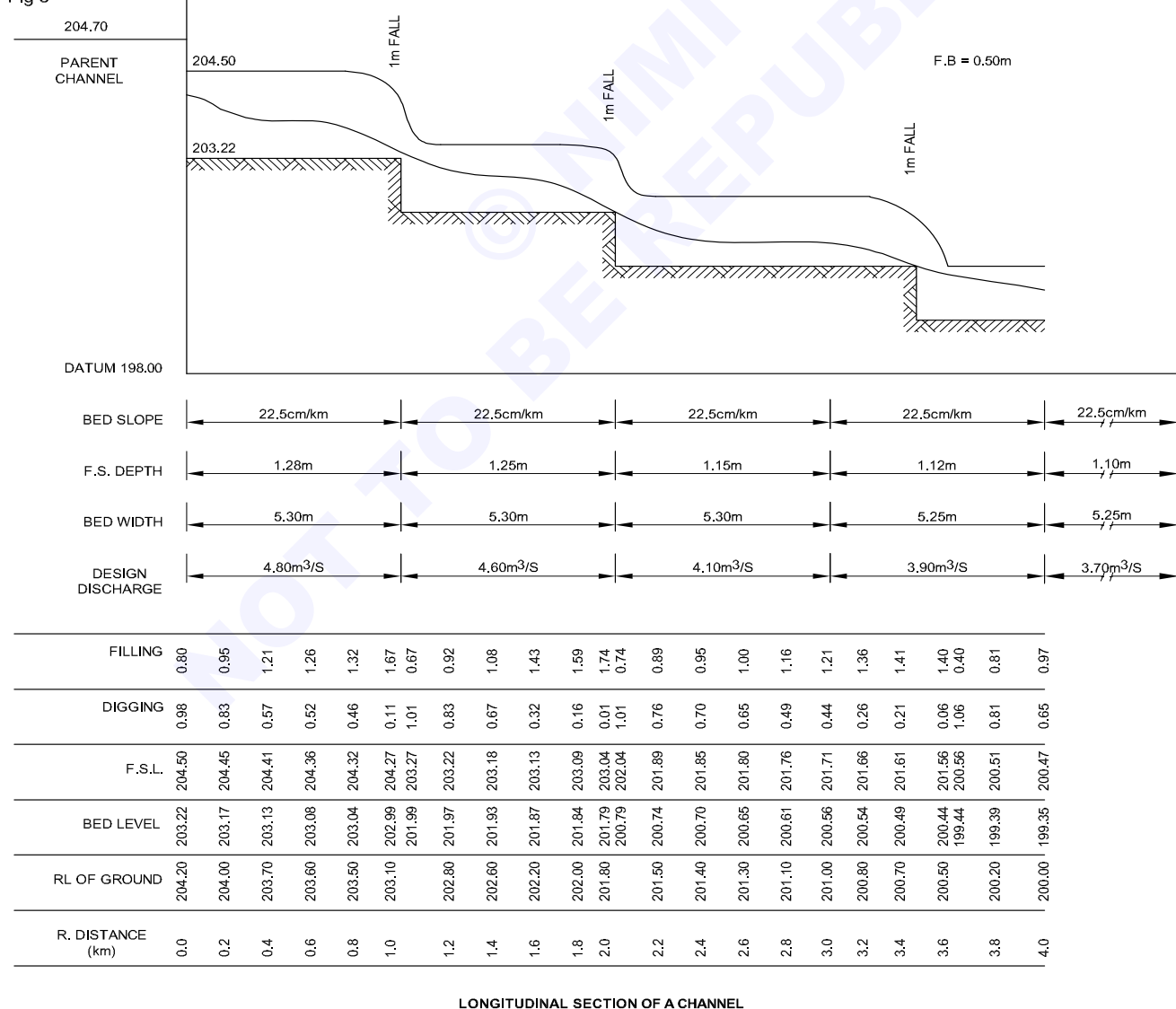
LONGITUDINAL SECTION OF A CHANNEL
