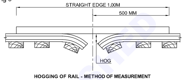
HOGGING OF RAIL - METHOD OF MEASUREMENT
