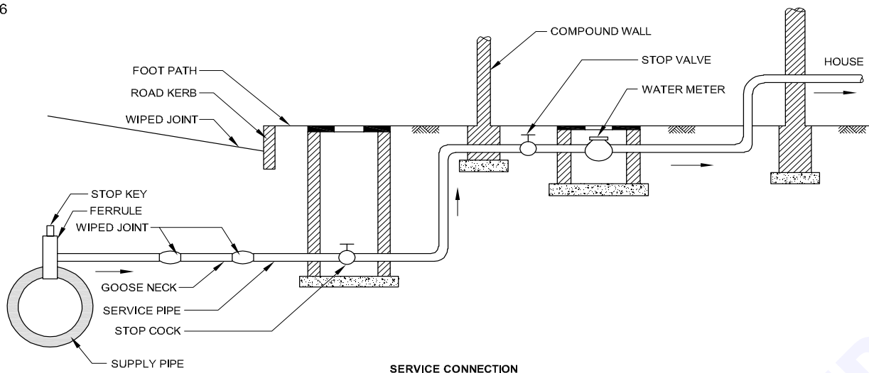
SERVICE CONNECTION
