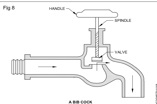
A BIB COCK
